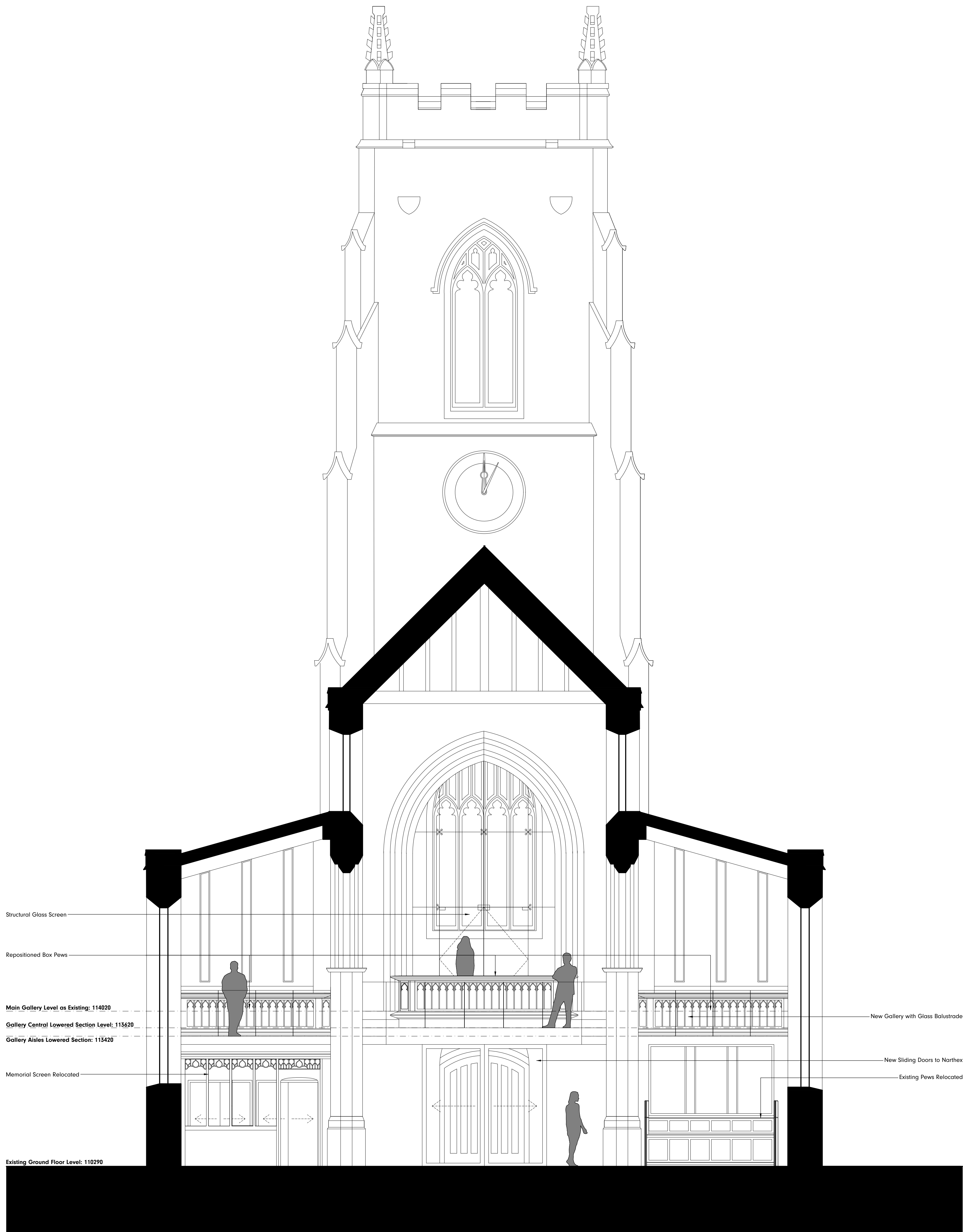
Proposed Section B 1:50
