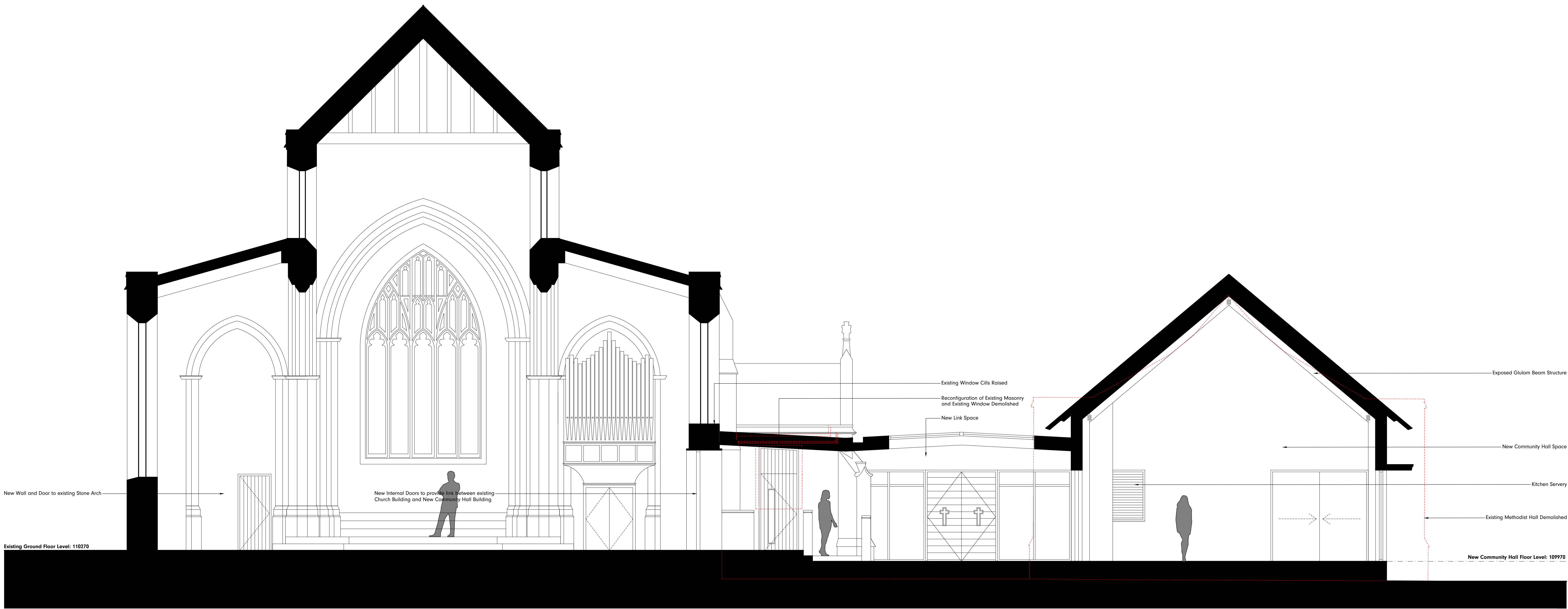
Proposed Section D 1:50
